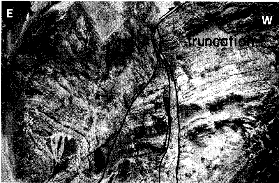
Fig. 5. Northern cliff of the Croda del Vallon Bianco, composed of Liassic Calcarei Grigi. The W-vergent basal thrust plane cuts a pre-existing (Liassic-Cretaceous?) normal fault. Note the cataclastic fault rock.
